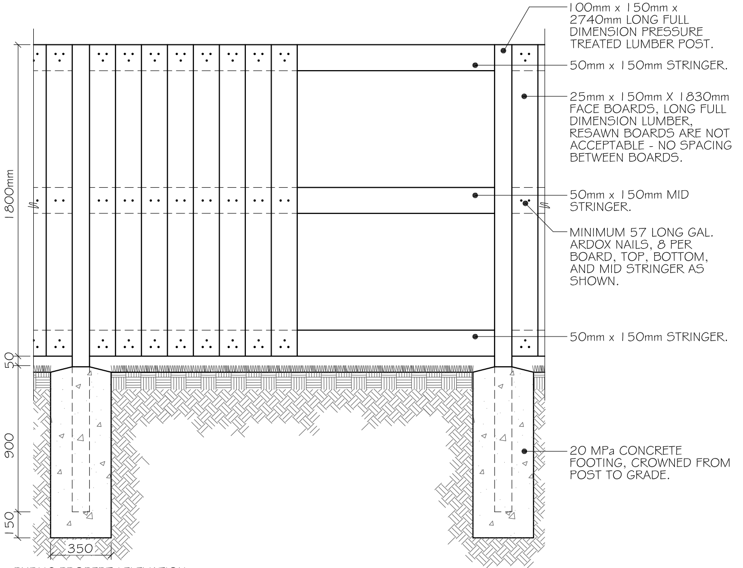
PUBLIC PROPERTY ELEVATION
